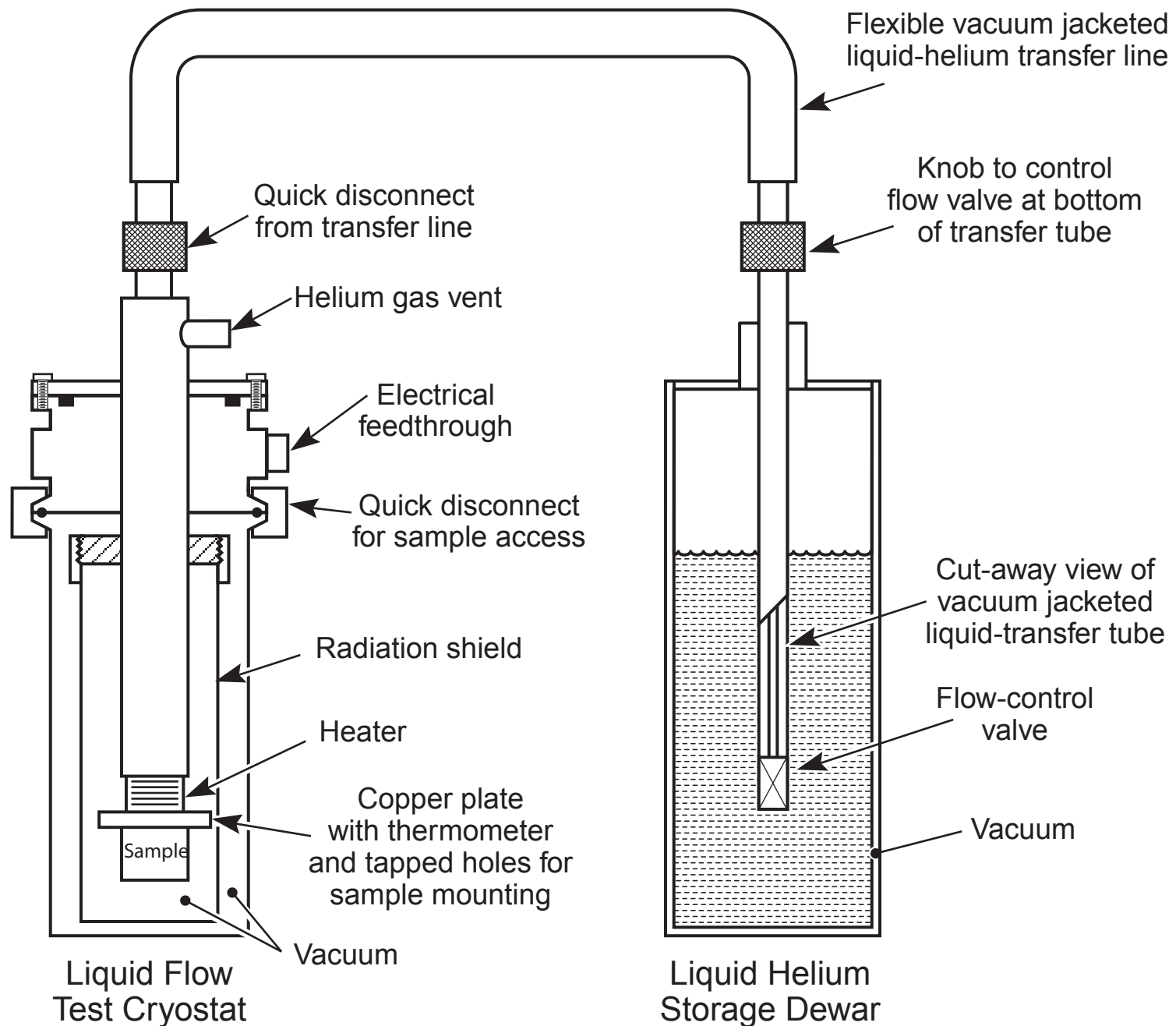
FIG. 1.10 Variable-temperature cryostat based on continuous transfer of liquid-cryogen from a storage dewar to a cold plate on which the test sample is mounted. Typically, the sample is situated inside an evacuated can, which is surrounded by a thermal radiation shield (figure modeled after one from a catalogue of Cryo Industries 2002).
