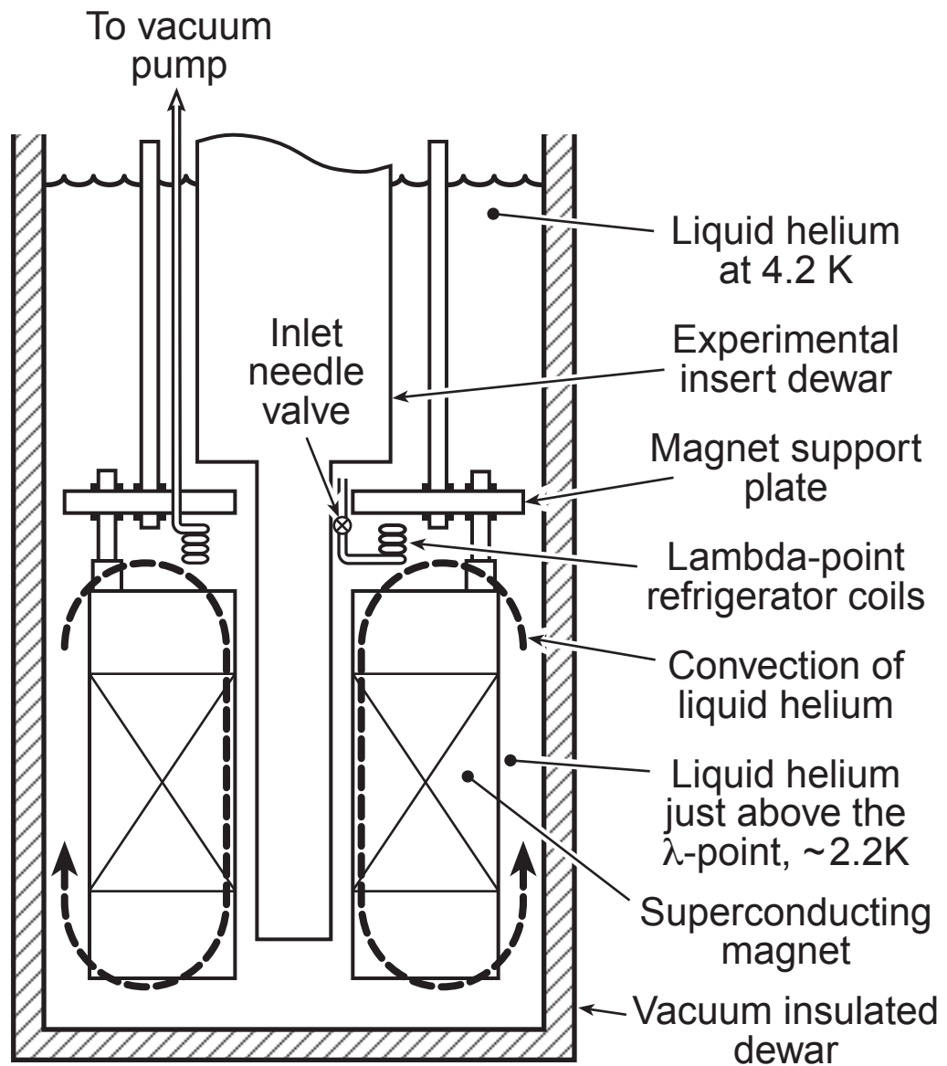
Lambda-Point Refrigerator
