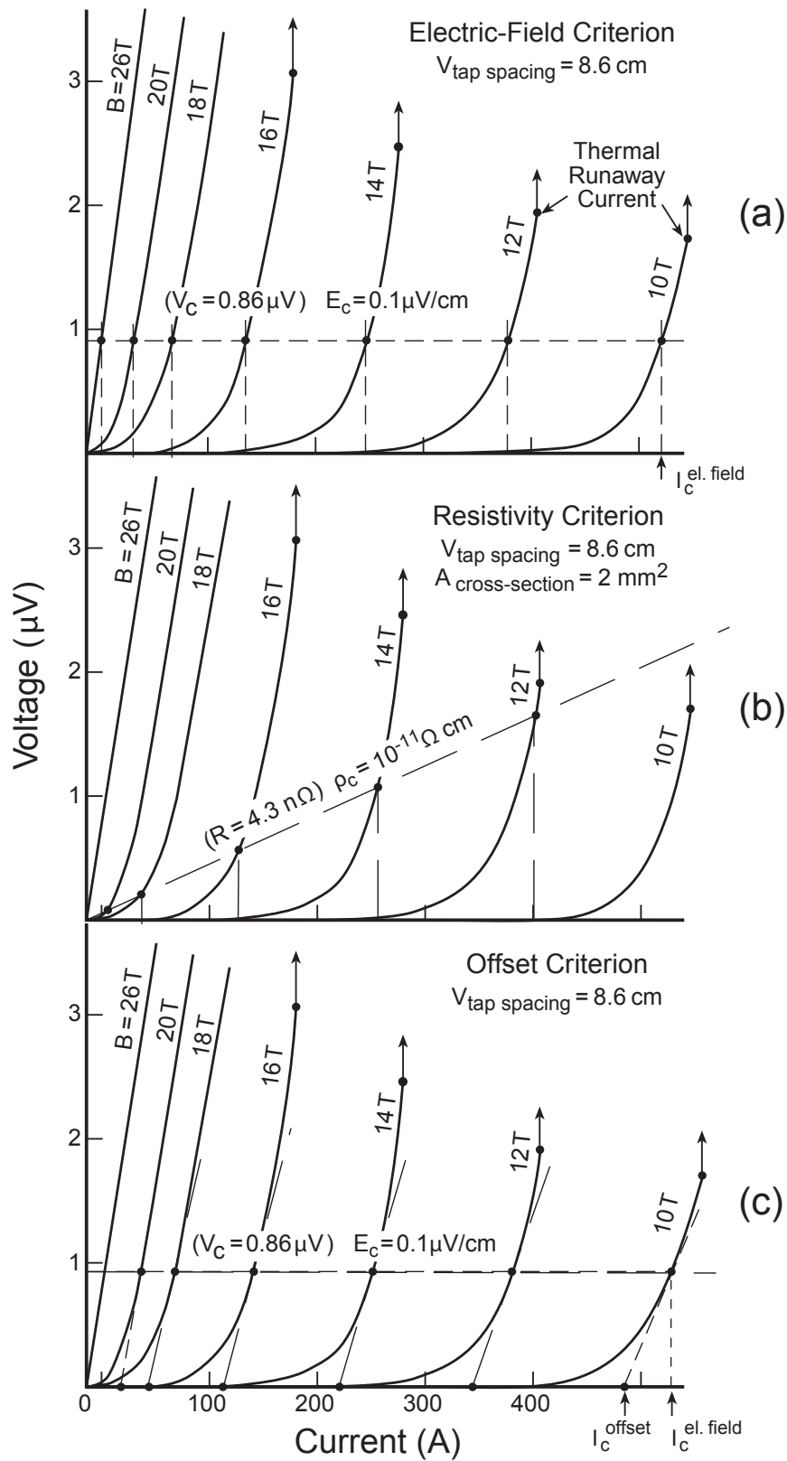
FIG. 10.1 Methods for determining the critical current from a set of V - I curves obtained at different magnetic fields: (a) electric-field criterion, (b) resistivity criterion, and (c) offset criterion (adapted from Ekin 1989).
