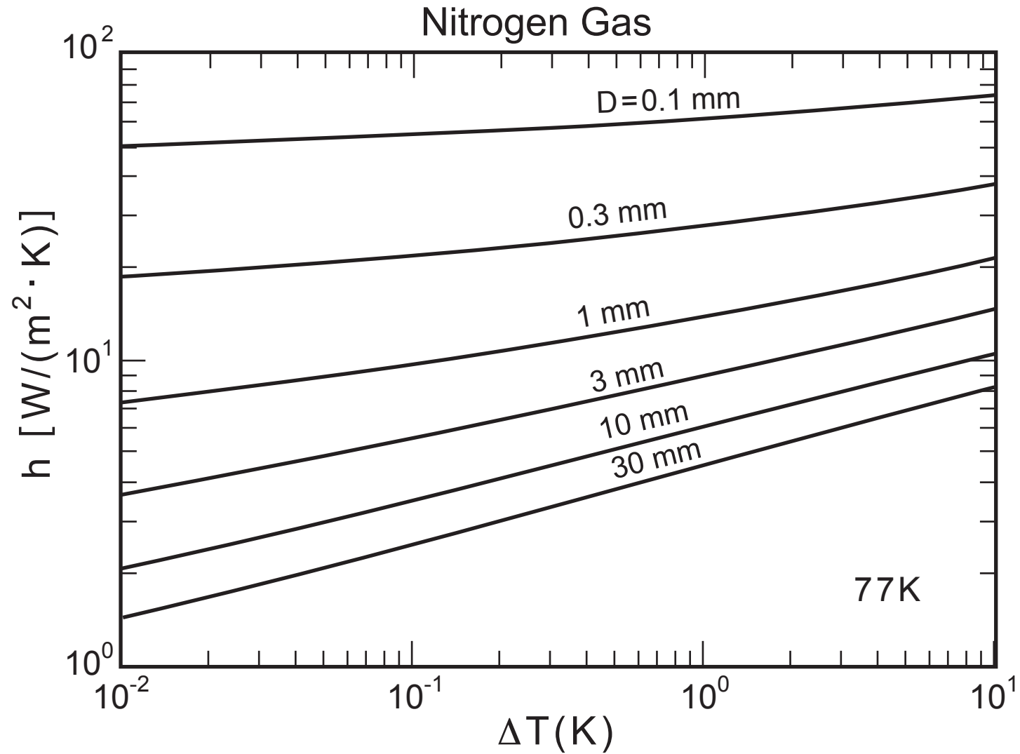
FIG. 2.10 Free-convective heat-transfer coefficient h between nitrogen gas and horizontal cylindrical solids of diameter D at 77\text{ K} , for use with Eq. (2.15). (Calculated by Marquardt 2002 from free-convection correlation data for fluids and gases compiled by McAdams 1954 and reproduced by Kreith and Bohn 2001.)
