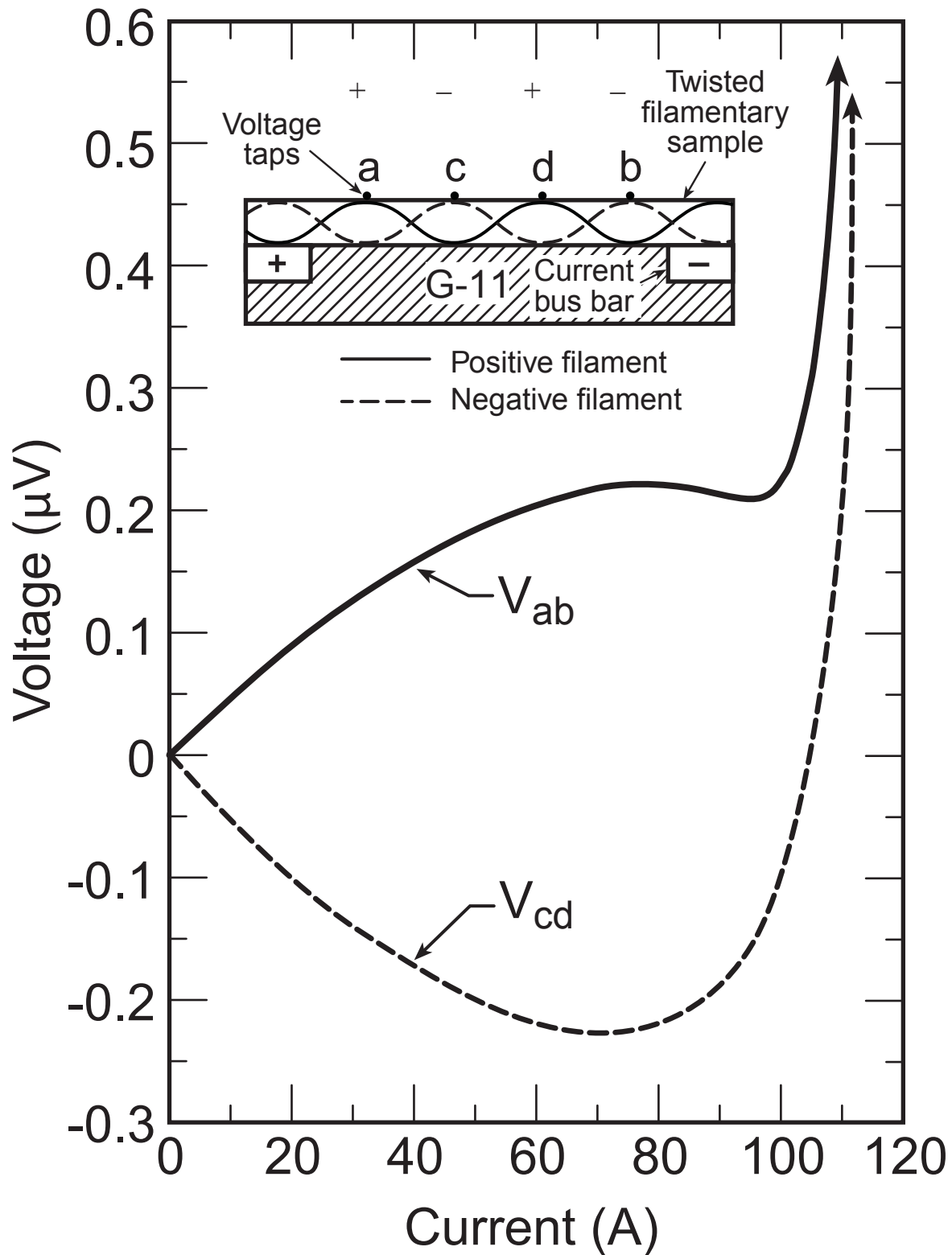
FIG. 7.12 Anomalous V - I characteristic of a short Nb-Ti sample, where the length of the current contact is less than a full twist pitch and there is an odd half-integer number of filament twists between the current contacts (from Goodrich et al. 1982).
