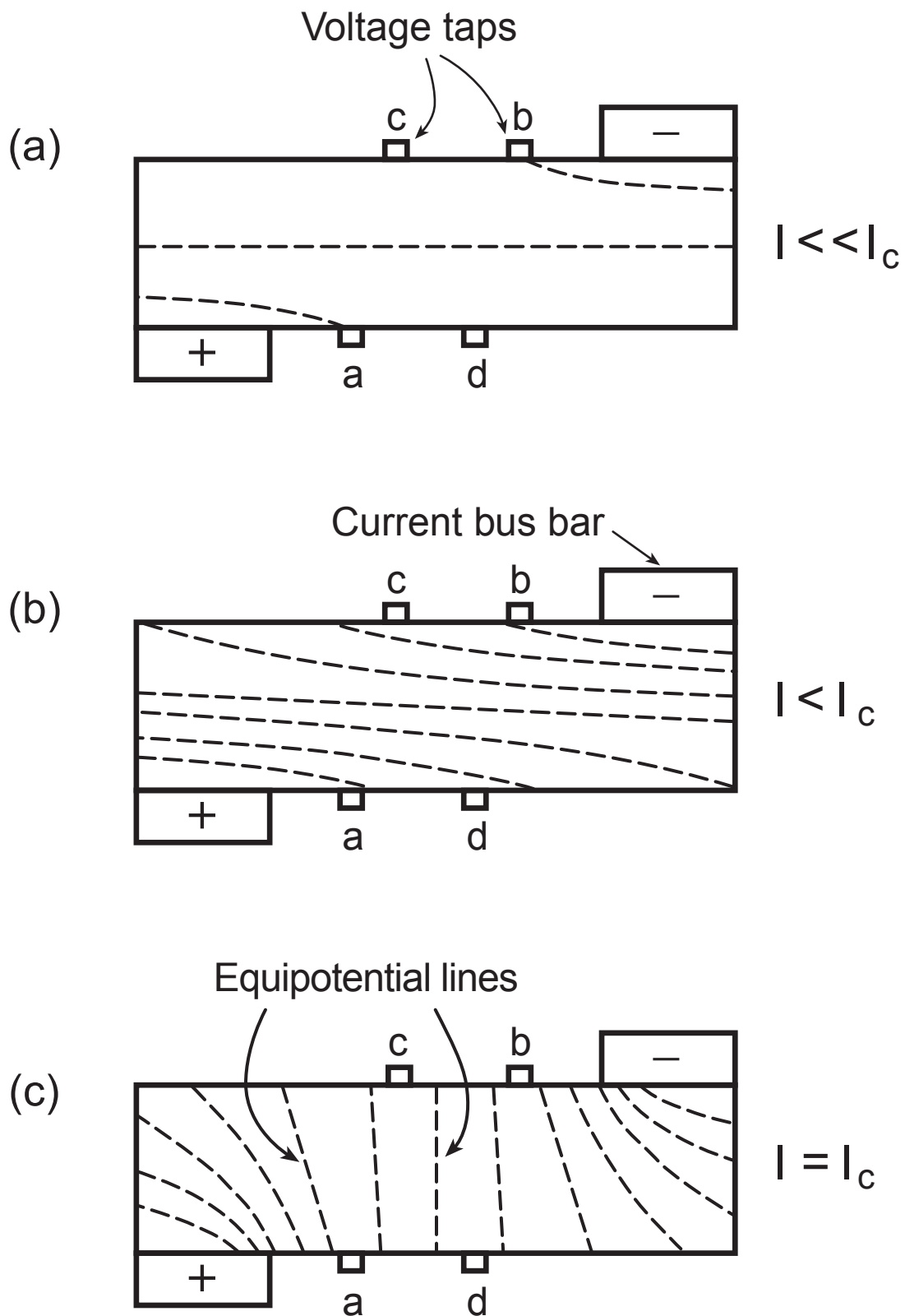
FIG. 7.13 Model of equipotential lines (dashed) for the superconductor test setup and data shown in Fig. 7.12: (a) current much less than I_c ; (b) intermediate currents less than I_c ; and (c) current near I_c . (Adapted from Goodrich et al. 1982.)
