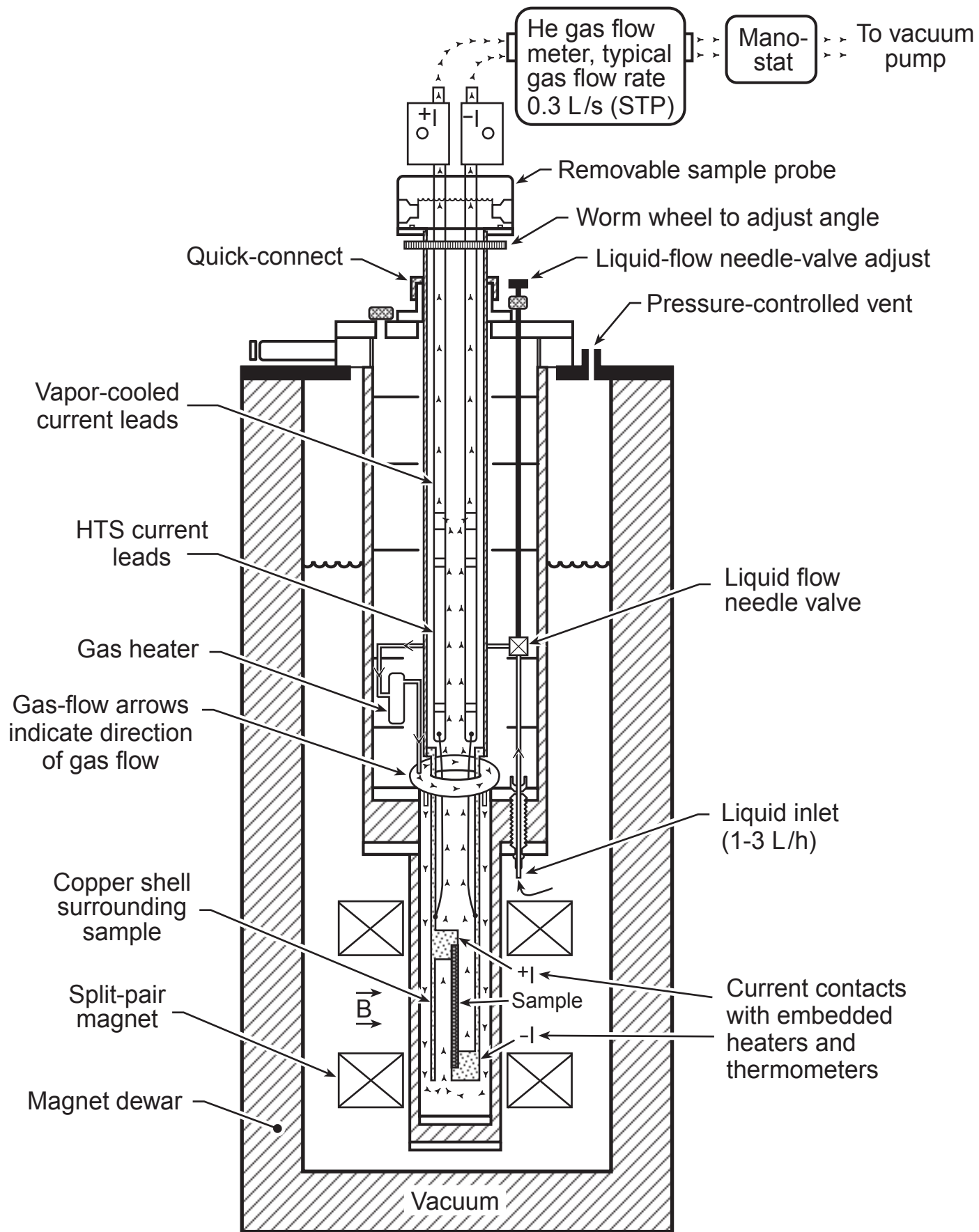
FIG. 9.13 High-current helium-gas-flow cryostat for measuring critical current at variable temperature and magnetic-field angle (from Goodrich and Stauffer 2001).
