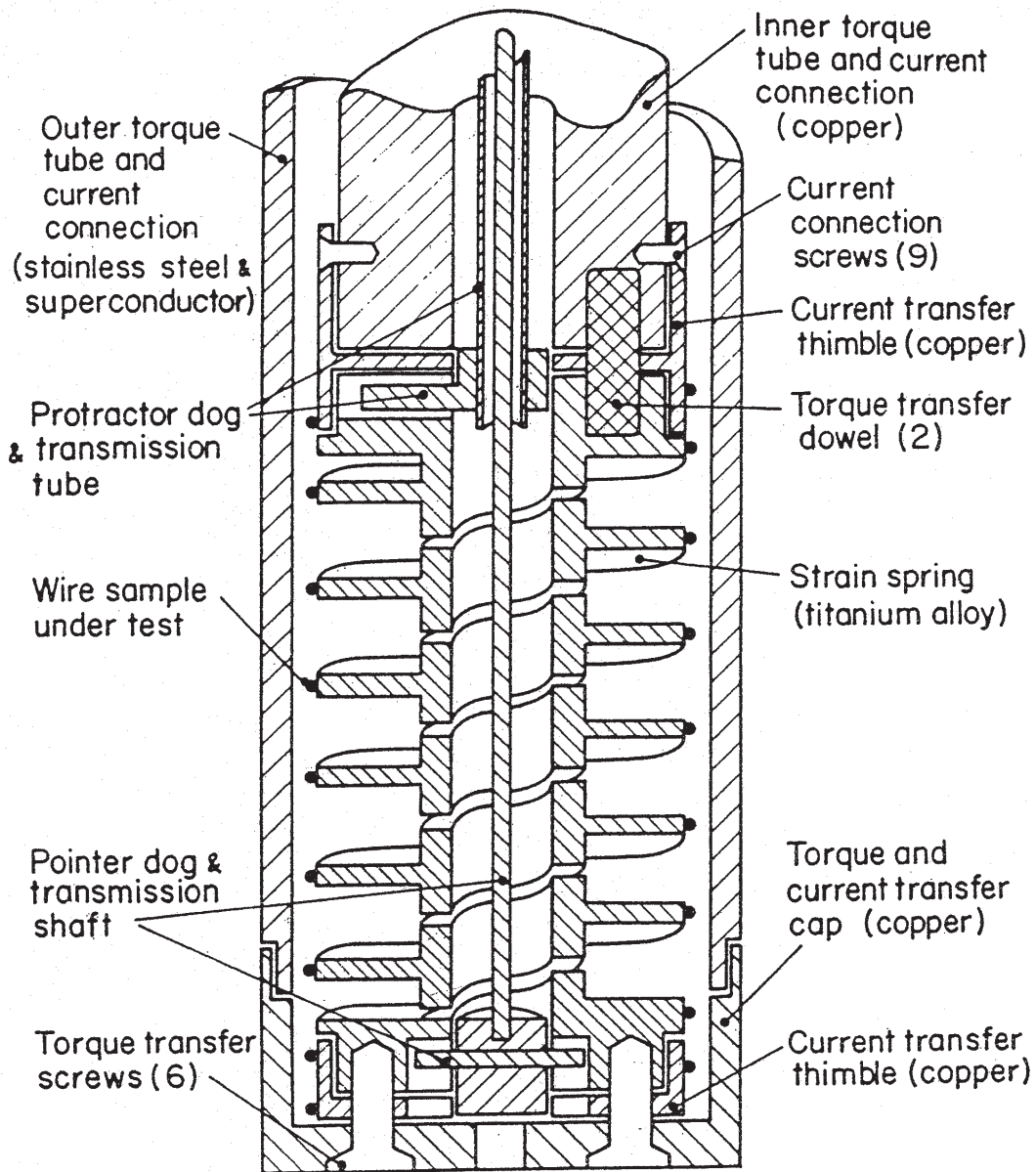
FIG. 9.15 Coil sample holder for measuring the effect of strain on the critical current of long superconductor samples (from Walters et al. 1986). The sample is soldered to a spring, which is twisted and untwisted through small angles to apply axial strain to the superconductor. Sample strain is measured by the angle of rotation of the coil.
